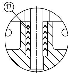
SHOWN WITH OPTIONAL TFE V-RING PACKING
